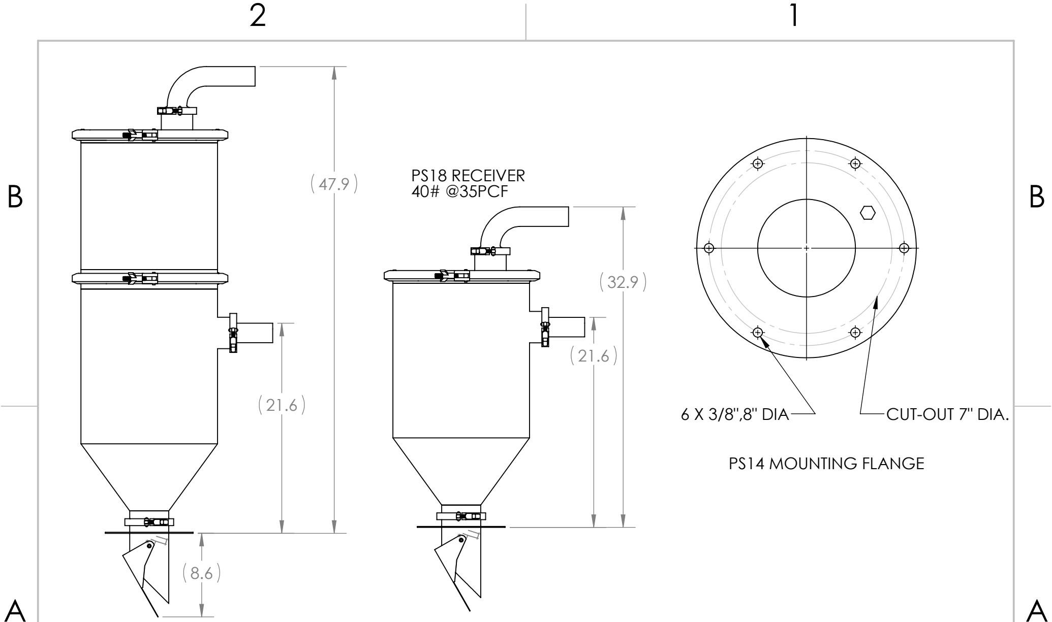
PS14 WITH BAG FILTER
